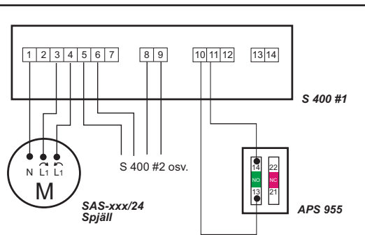
Schema APS 955
