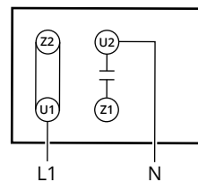
Driftkondensator, (motsols rotation)
